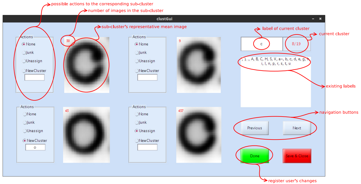
Figure 4: Graphical User Interface.
